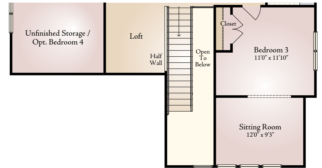
Partial Upper Level Floor Plan Elevation 3
