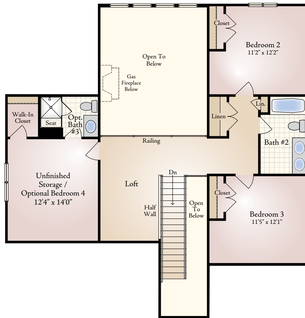
Partial Upper Level Floor Plan Elevations 1 and 2
