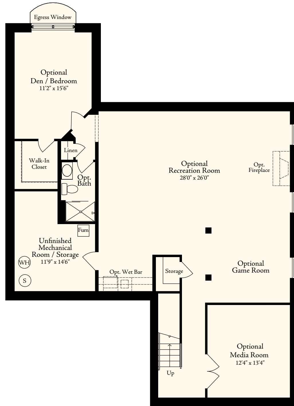
Lower Level Floor Plan Elevations 1, 2, and 3
