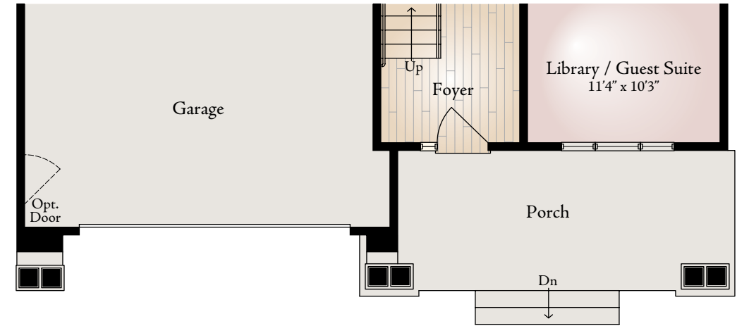
Partial Main Level Floor Plan Elevation 3
