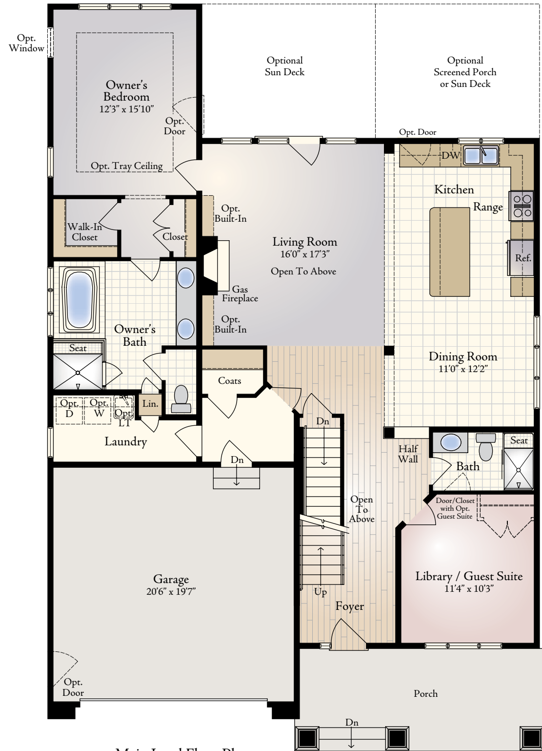
Main Level Floor Plan Elevation 1
